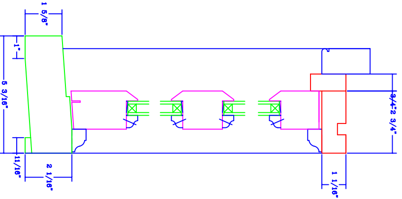
HEAD DETAIL TYPICAL
