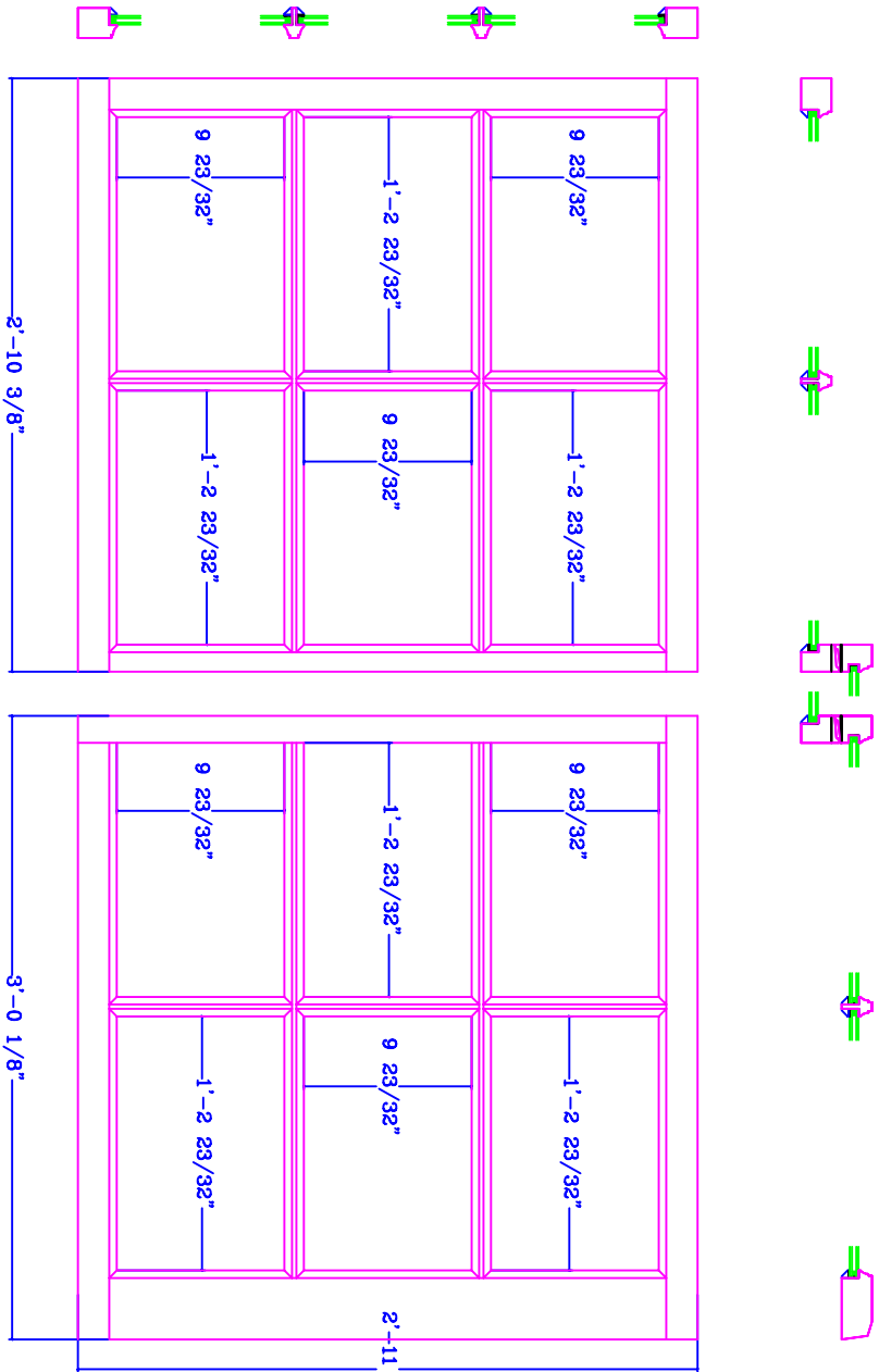
ELEVATION - MOCK-UP SCALE: 3/8" = 1'
